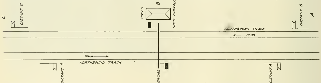
TYPICAL ARRANGEMENT OF TOWER, SIGNAL BRIDGE AND SIGNALS. MANUAL CONTROLLED SYSTEM. N. Y. C. & H. R. R. R.
